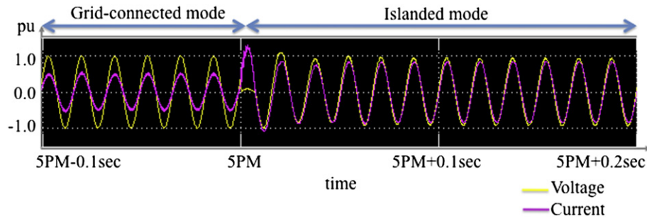
Fig. 8. The variation of 60 Hz voltage and current waveforms measured at the interconnection point before and after the upstream outage applied to the circuit.
